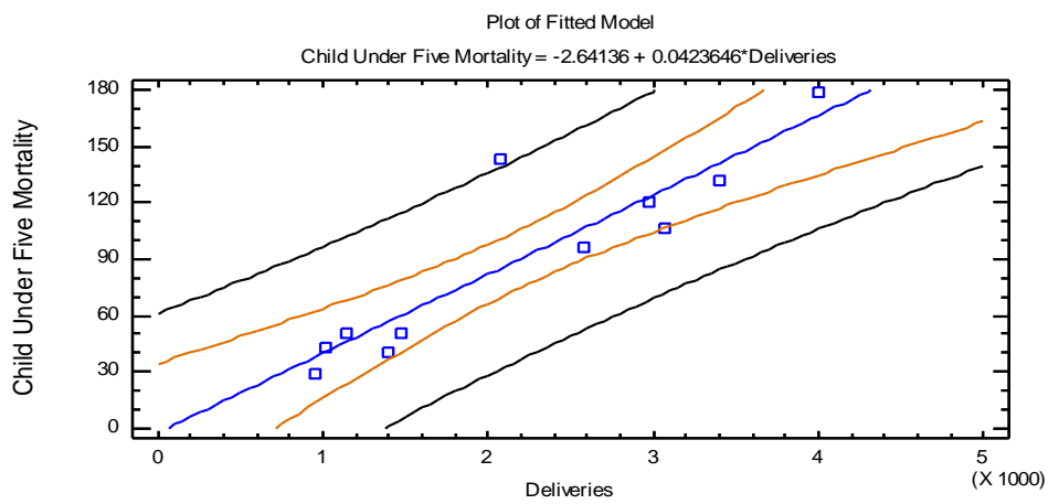
Figure 2: Simple Regression - Infant and Child Mortalities vs. Deliveries
