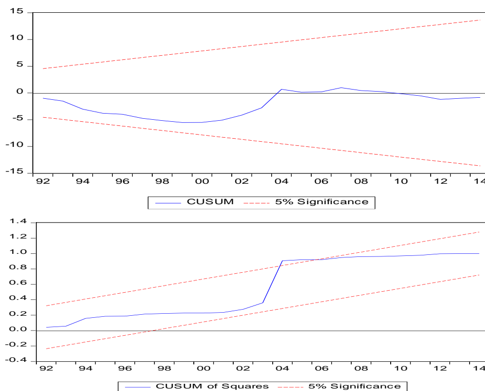
Figure 2 plot of CUSUM and CUSMQ for the coefficient stability of ECM model \Delta \ln rgdpc
